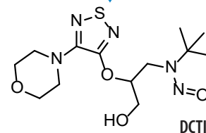
NDSRI of Timolol Impurity B
