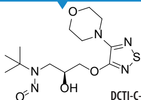
N-Nitroso Timolol
