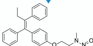
N-Nitroso Desmethyl Tamoxifen (Mixture of isomers)
