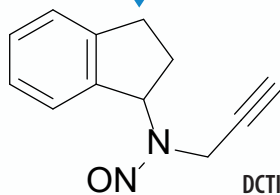
N-Nitroso Rasagiline
