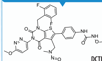
Relugolix nitroso impurity
