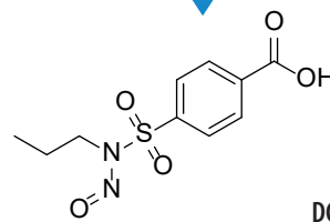
4-(N-nitroso-N-propylsulfamoyl) benzoic acid
