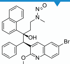
N-Nitroso-N-Desmethyl Bedaquiline
