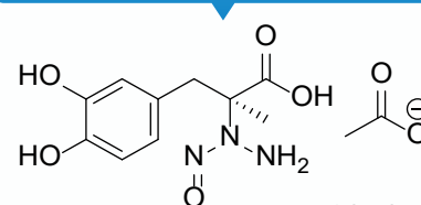
N-Nitroso Carbidopa Acetate Salt
