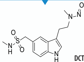
N-Nitroso-Desmethyl-Sumatriptan Impurity
