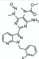
Riociguat Nitroso USP Related Compound C
