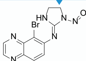
N2-Nitroso Brimonidine
