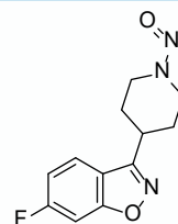
6-fluoro-3-(1-nitrosopiperidin-4-yl) benzo[d]isoxazole
