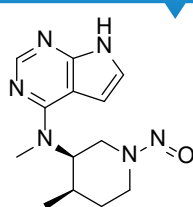
Tofacitinib Nitrosoamine Impurity-1
