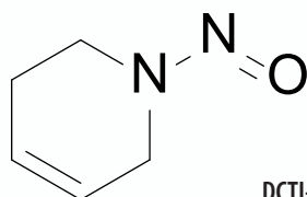
1-nitroso-1,2,3,6-tetrahydropyridine
