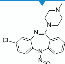
N-Nitroso Clozapine
