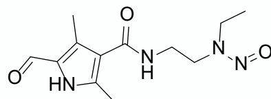
N-(2-(ethyl(nitroso)amino)ethyl)-5-formyl-2,4-dimethyl-1H-pyrrole-3-carboxamide
