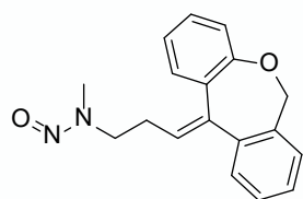
N-Nitroso-Desmethyl-Cidoxepin
