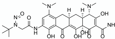
N-Nitroso Tigecycline
