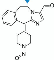
N-Nitroso Apixaban Ring Open Acid Impurity
