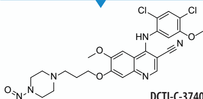
Bosutinib Nitroso Impurity
