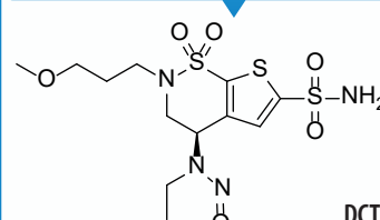
Brinzolamide Nitroso Impurity
