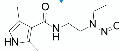
N-(2-(ethyl(nitroso)amino)ethyl)-2,4-dimethyl-1H-pyrrole-3-carboxamide
