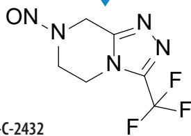
7-nitroso-3-(trifluoromethyl)-5,6,7,8-tetrahydro-[1,2,4]triazolo[4,3-a]pyrazine
