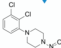
1-(2,3-dichlorophenyl)-4-nitrosopiperazine
