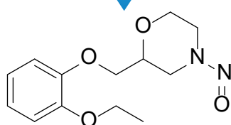
N-Nitroso Viloxazine
