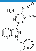
Riociguat Nitroso Impurity-1
