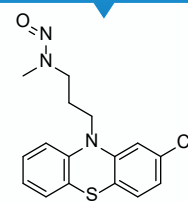
N-Nitroso Desmethyl Chlorpromazine
