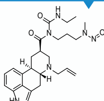
N-Nitroso Desmethyl Cabergoline
