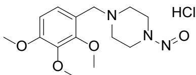
N-Nitrosamine Trimetazidine.HCl
