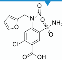
NDSRI of Furosemide impurity-A
