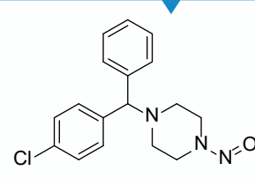
1-(4-chloro-benzhydryl)-4-nitrosopiperazine
