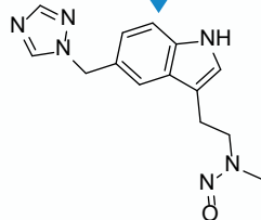
N-Nitroso Desmethyl Rizatriptan
