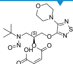
NDSRI of Timolol Related Compound E
