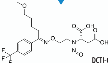
N-Nitroso Fluvoxamine EP Impurity C
