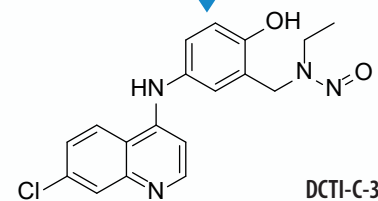
N-Nitroso N-Desethyl Amodiaquine
