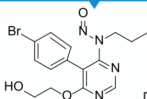
hydroxy N-nitroso n-propyl impurity
