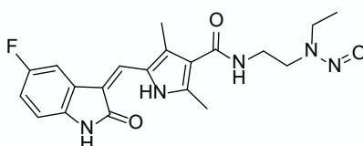
(Z)-N-(2-(ethyl(nitroso)amino)ethyl)-5-((5-fluoro-2-oxoindolin-3-ylidene)methyl)-2,4-dimethyl-1H-pyrrole-3-carboxamide
