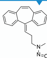
N-nitroso Cyclobenzaprine
