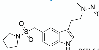
N-nitroso-Desmethyl-Almotriptan
