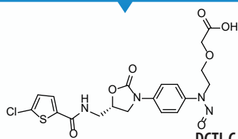
N-Nitroso Rivaroxaban Open-Ring Acid Impurity
